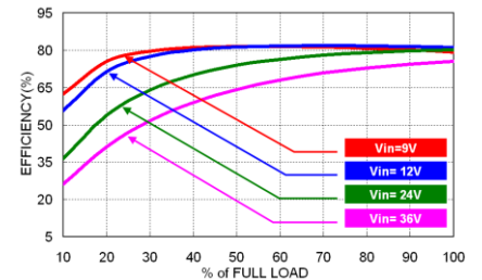
EDL03-24S05W Efficiency vs. Output Load
