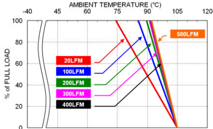
EDL03-24S05W Derating Curve
